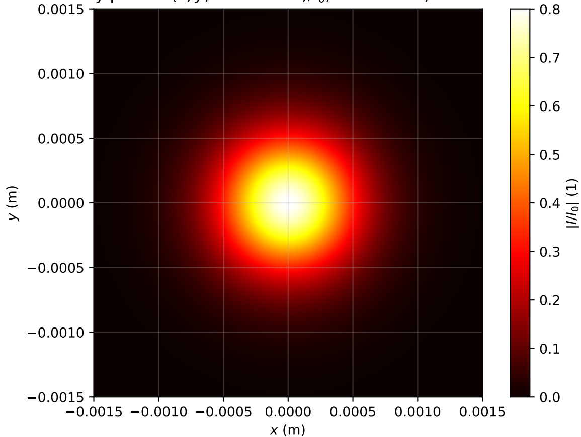
Intensity profile I(x, y, z = 1.751m)/I_0 , \text{Pin}=0.4\text{Pcr} , artificial time
